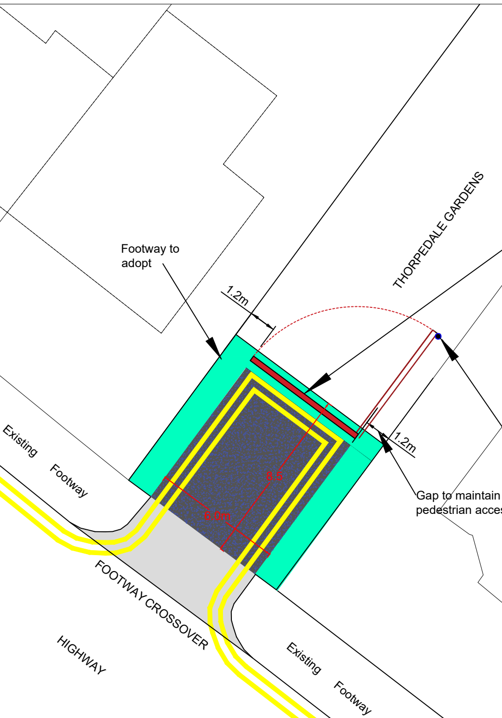
THORPEDALE GARDENS - TYPICAL ADOPTION PLAN and ACCESS GATE
